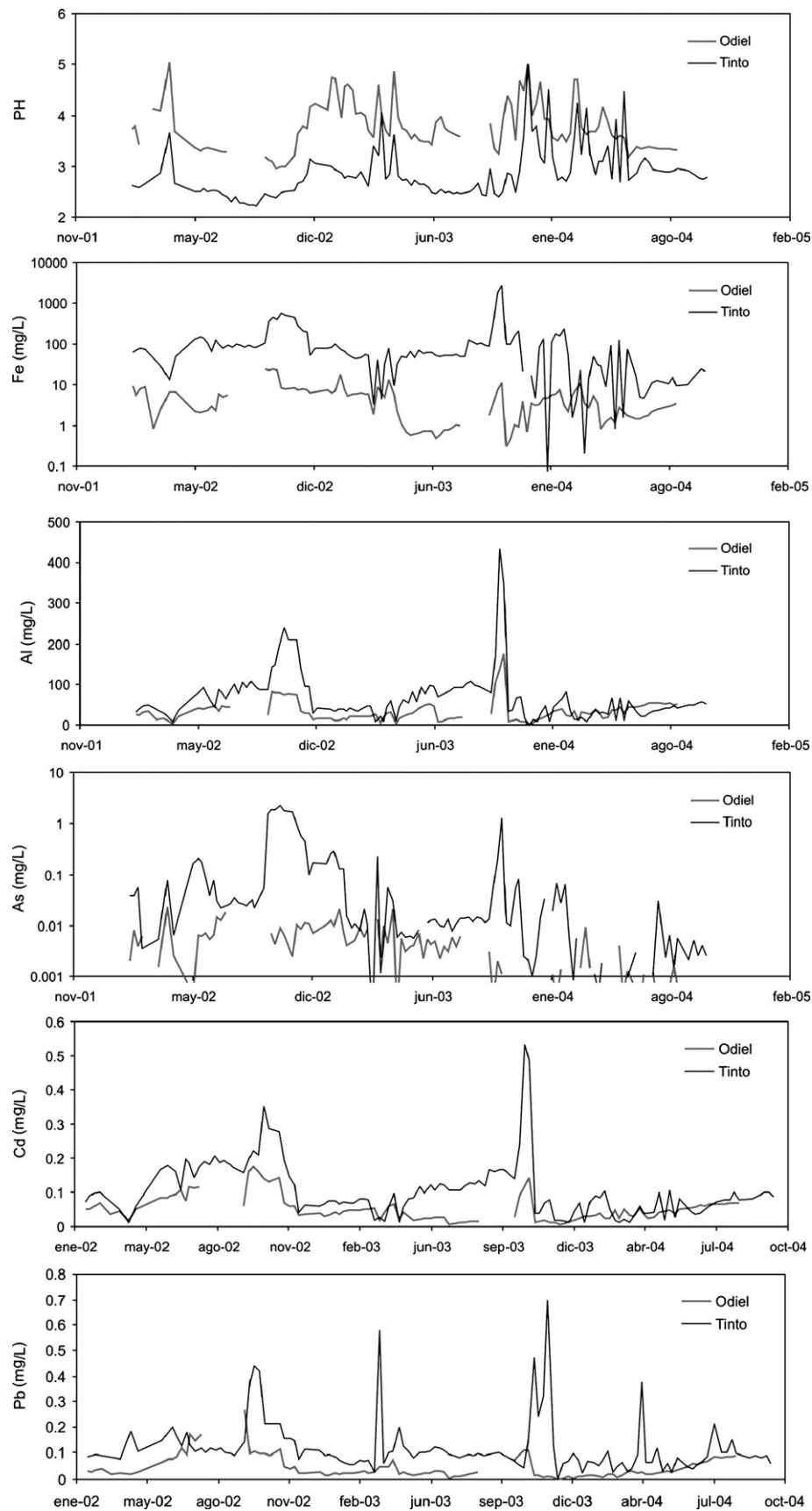
Fig. 3. Evolution of pH and Fe, Al, As, Cd and Pb concentration in the Tinto and Odiel rivers from February 2002 to September 2004.
