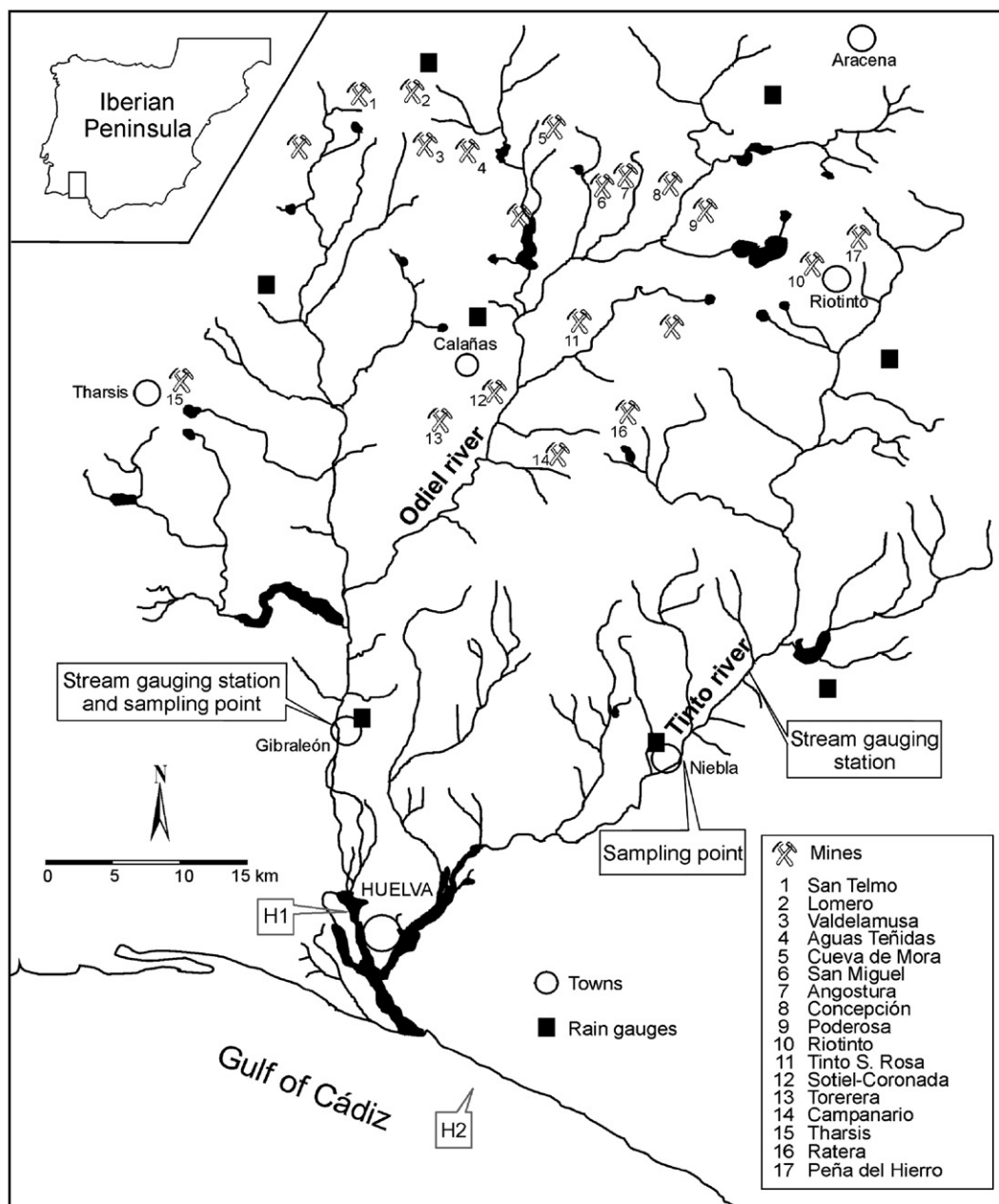
Fig. 1. Sketch map of the Tinto and Odiel rivers, showing the location of the sampling points, stream gauging stations, rain gauges, and main mine localities.
