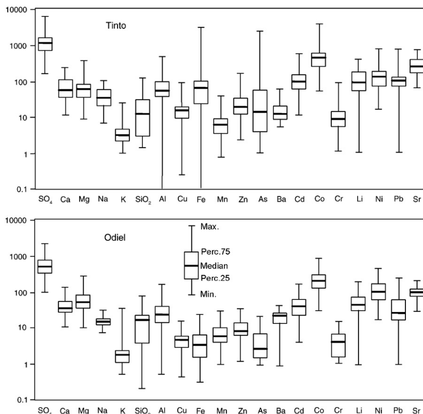
Fig. 2. Box and whisker plot of the dissolved elements in the Tinto and Odiel rivers (values in mg/L except for As, Ba, Cd, Co, Cr, Li, Ni, Pb and Sr which are in \mu\text{g/L} ).
