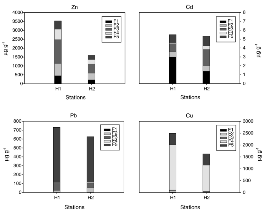
Fig. 5. Trace metal distribution in the five geochemical fractions of the sediment collected from the Huelva estuary. Results are expressed as µg/g dry sediment. Sediments collected in station H1 are in the fresh water area of influence of the estuary, whereas sediments located in H2 are in the sea water area of influence of the estuary.
