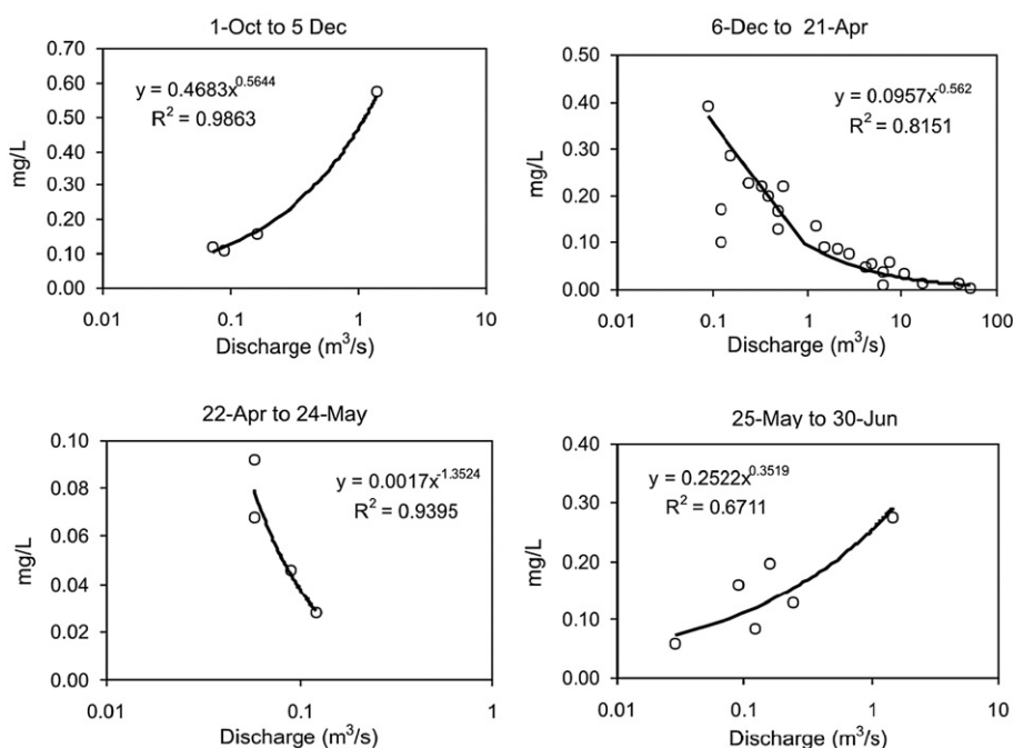
Fig. 4. Relationships Cd-discharge in the Tinto river for the different periods used for the contaminant load calculation (hydrological year 1996/1997).
