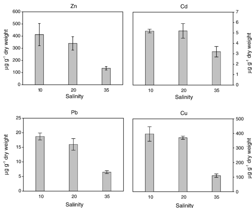
Fig. 7. Histogram of summarized results of trace metal concentration analyzed in tissues of clams Ruditapes philippinarum exposed to sediments collected from the Huelva estuary at three salinity values (10, 20 and 35). Results are expressed as microgram per gram of dry weight.
